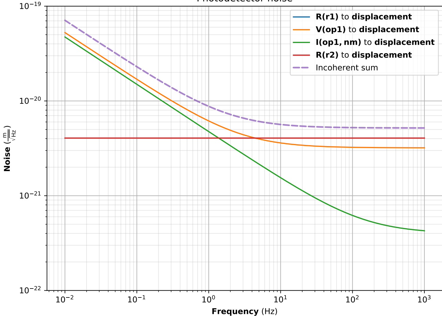
Photodetector noise
